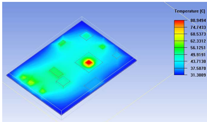
Figure 10: Effect of copper percentage on board
