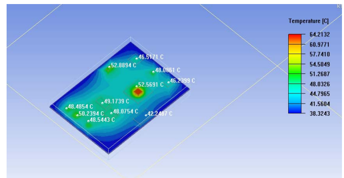
Figure 8: temperature distribution at normal condition
