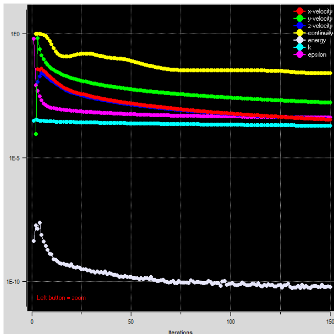
Graph1: Different CFD values for 150 iterations
