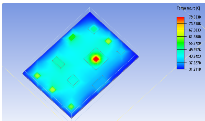
Figure 11: Effect of component placement on the board and components
