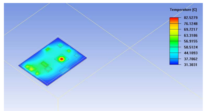
Figure 9: Temperature distribution of the board at loaded condition
