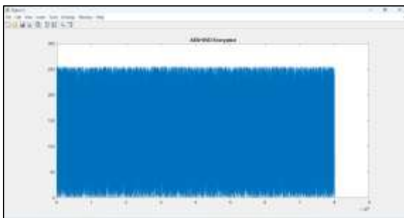
Figure 6: AES+SVD Encryption
