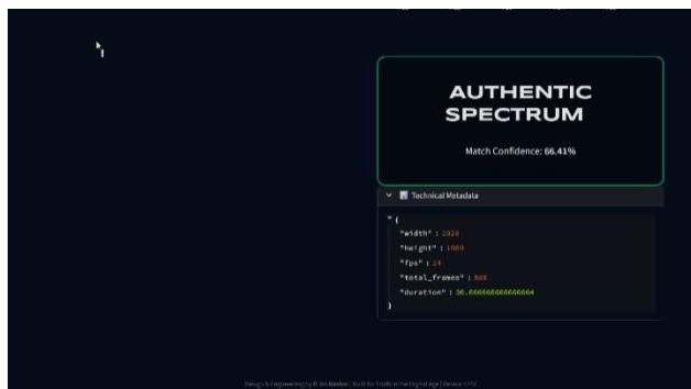
Fig. 3: Expected Results
