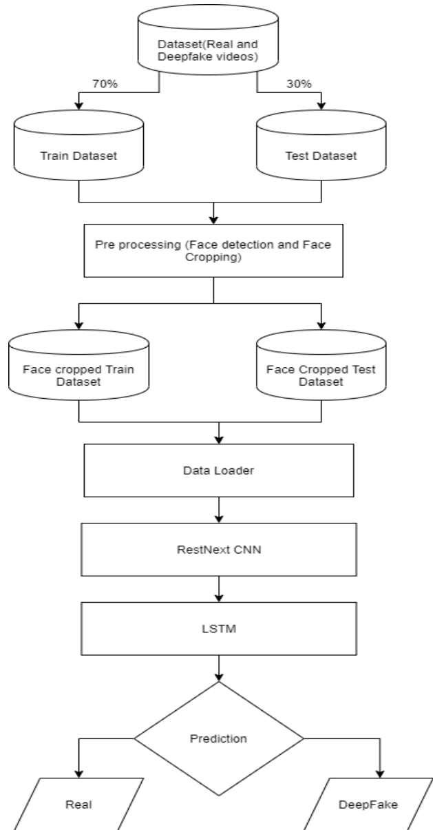
Fig. 2: Training Flow
