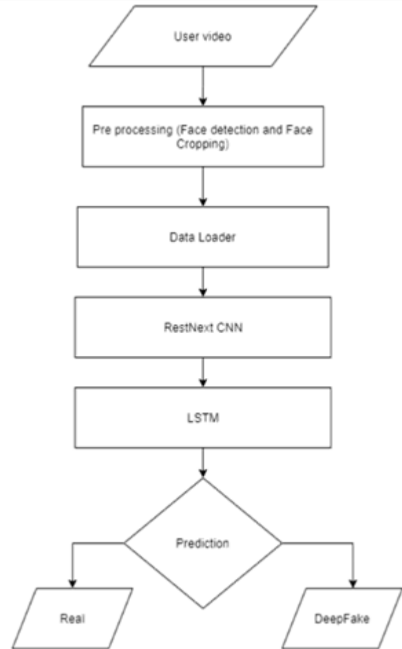
Fig. 4: Prediction flow
