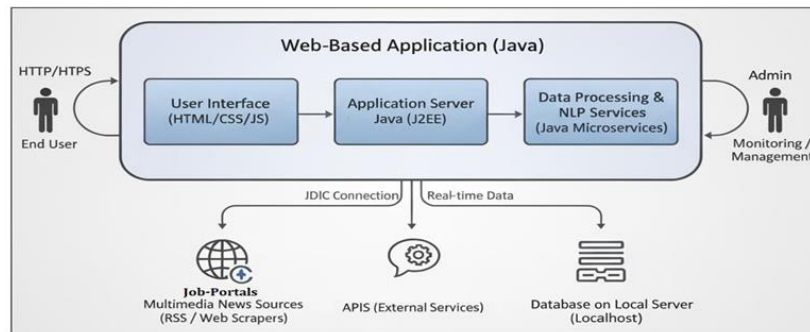
Fig.1: System Design
