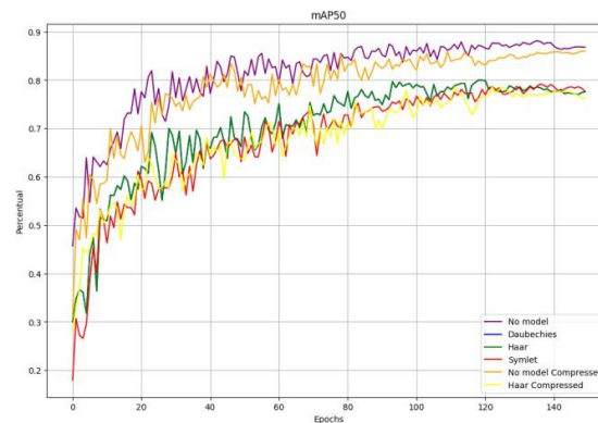
Fig 5 : mAP50 vs. Epochs for Different Models
