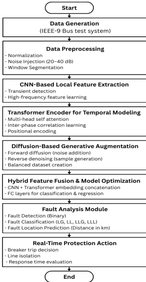
Figure 1: Proposed DET Hybrid Framework for Real-Time Fault Analysis
