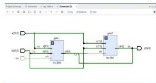
Fig. 4. RTL schematic of ALU before modification
