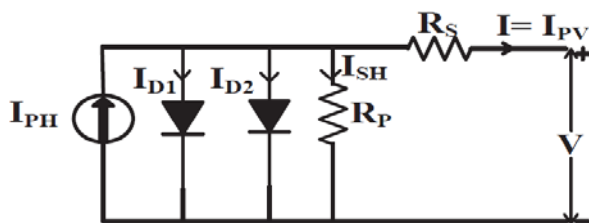
Fig. 2. Equivalent circuit of two-diode model of PV cell
