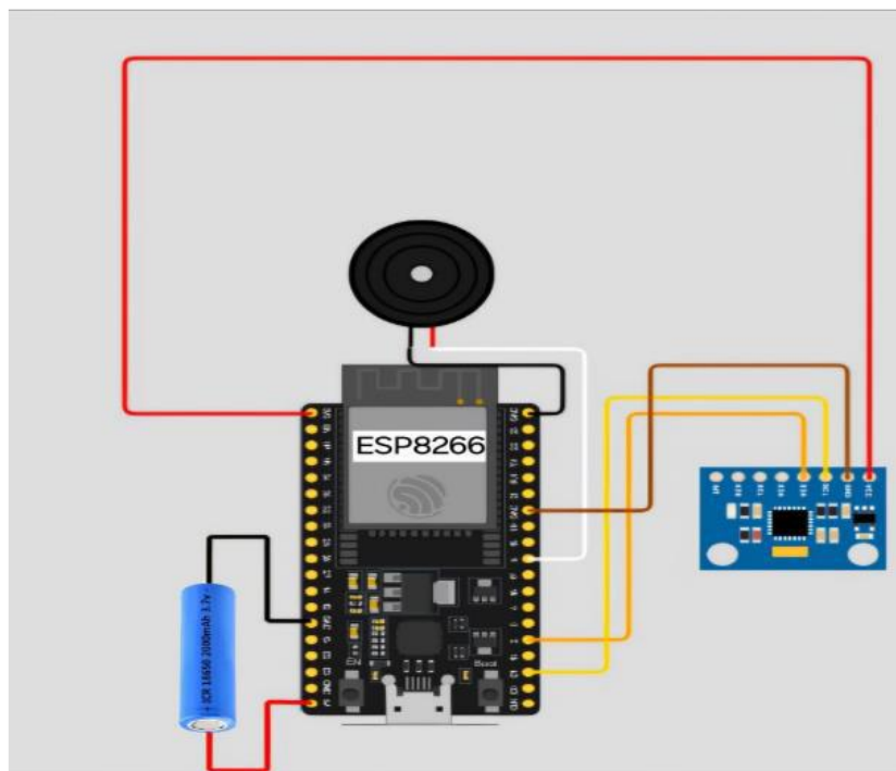
Fig 3. Circuit diagram showing components and connections
