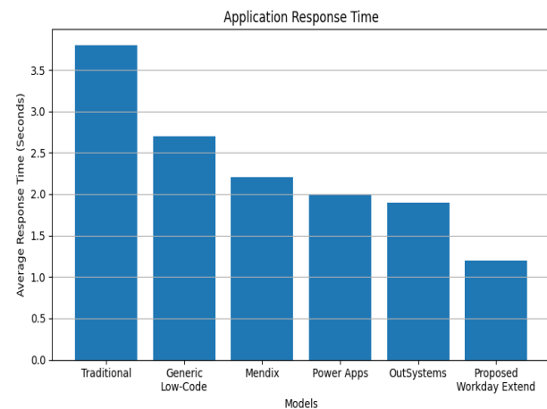
Fig. 5. Application Response Time
