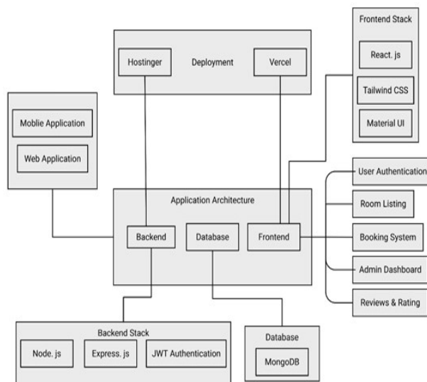
Figure:1 Model Architecture.
