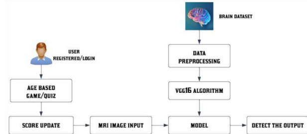
Fig 1. Architecture Diagram
