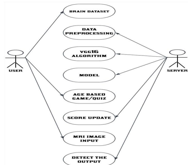
Fig.2 UML Diagram
