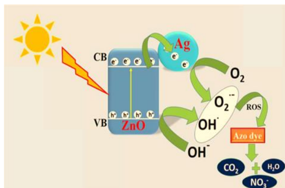
Fig:3 Formation of oxygen reactive species
