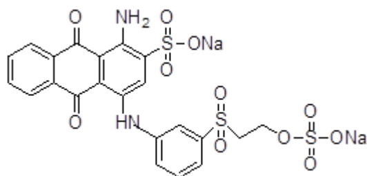
Chemical structure of Remazol Brilliant blue dye Azo dyes
