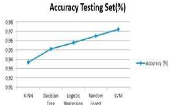
Fig.3. Comparative graph of different classifiers
