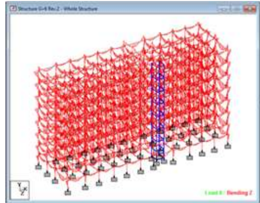
Fig.2 – Bending in Z Direction for Load Combination (1.5DL + 1.5LL)
