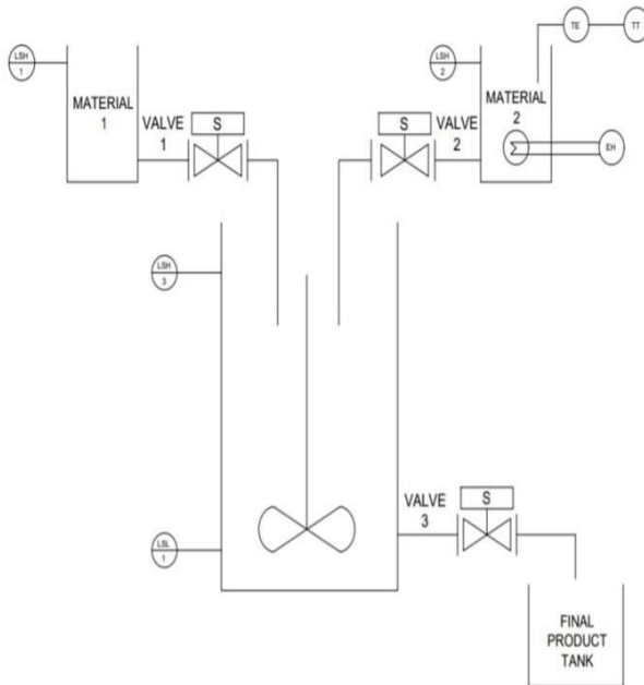
Figure 3: P&ID
