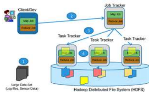
Fig. 1. MapReduce and HDFS
