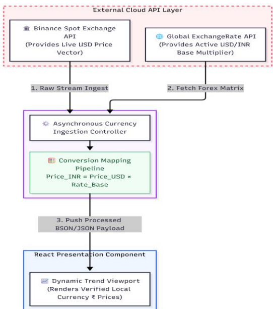
Fig. 4: Asynchronous External API Data Processing Flow and Currency Localization Stack.
