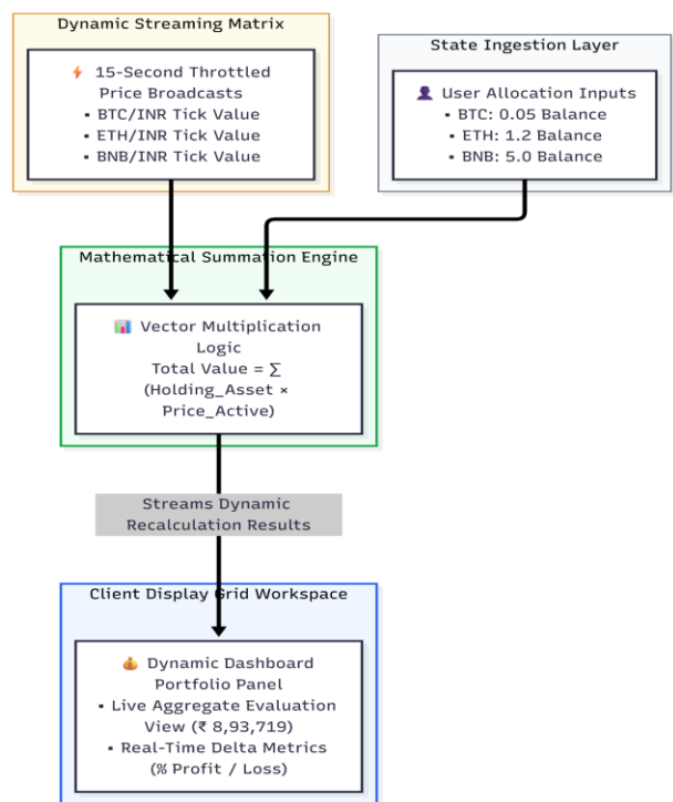
Fig.5: Personalized Asset Matrix Calculation and Rebalancing Engine Flow.
