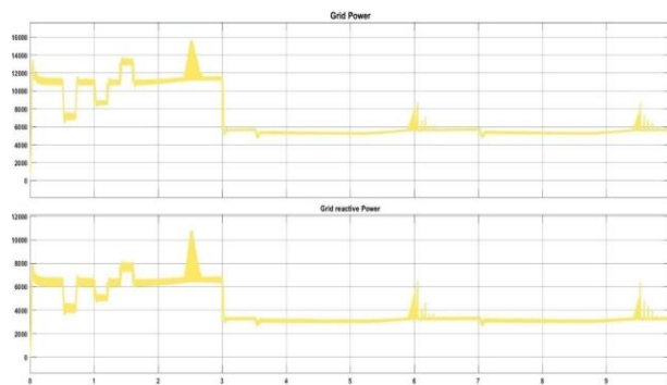
Fig. 9: Grid Power
