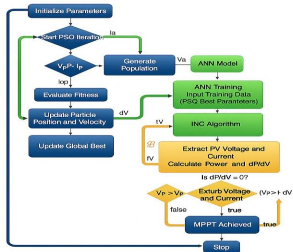
Fig. 3: Working flow chart of proposed MPPT
