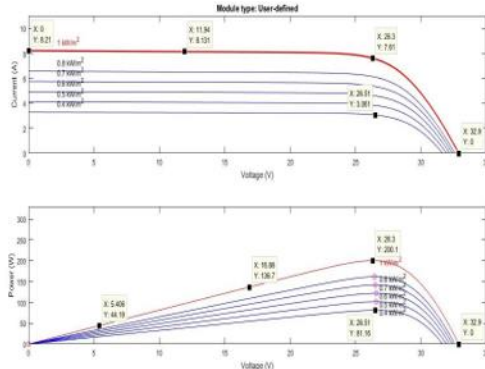
Fig. 2(b): Characteristics of PV module Fig.2: Elaboration of PV module
