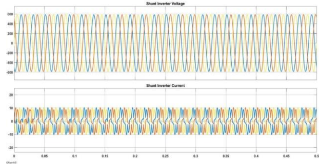
Fig. 8: Shunt inverter voltage and current
