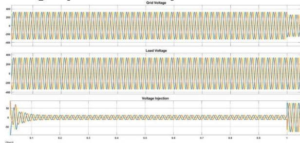
Fig. 11: Grid Voltage Injection
