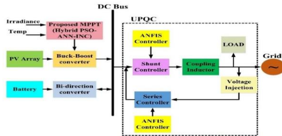
Fig.1: Block diagram of system
