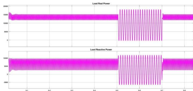
Fig. 12: Load Power
