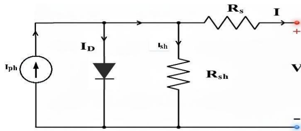
Fig. 2(a):PV model based on Mathematical equations
