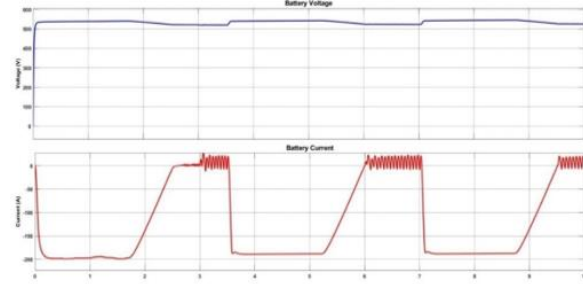
Fig. 4: Battery Output
