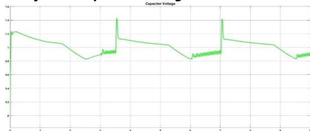
Fig.6: Capacitor Voltage
