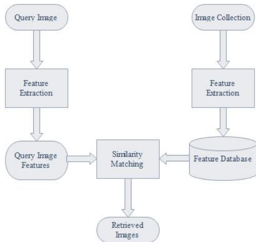
Fig. 1. Overview of Typical CBIR System.
