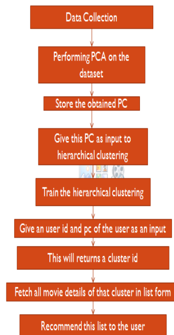
Fig.1. Flowchart for the proposed system.
