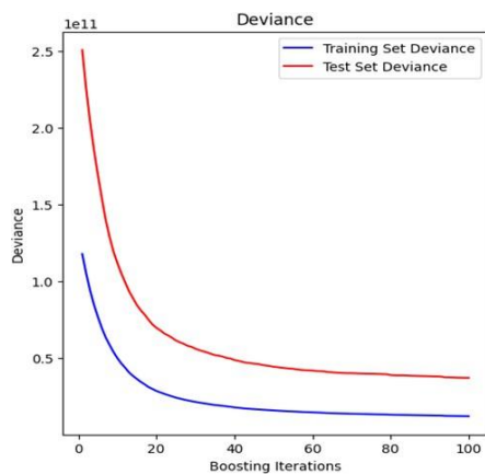
Chart - 4: A graph between the Deviance and Boosting Iterations
