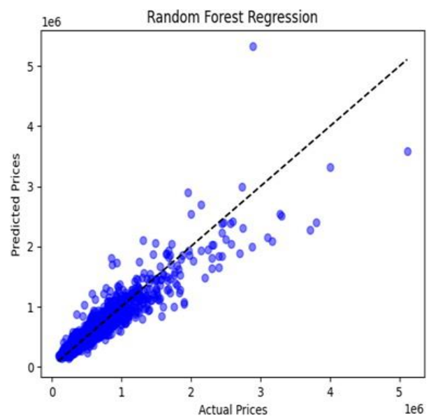
Chart - 1: Predicted Graph of Random Forest Regression Additionally, Random Forest has a proprietary
