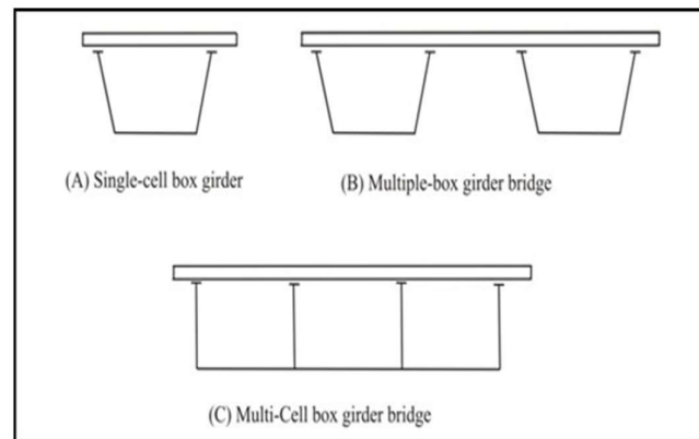
(A) Single-cell box grider (B) Multiple box grider bridge (C) Multi-cell grider bridge
