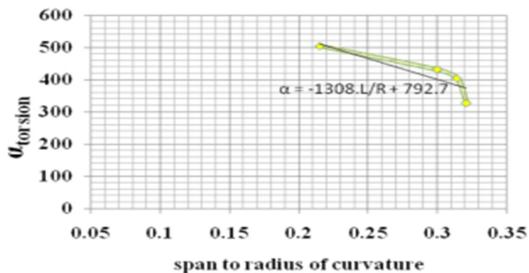
Figure 3: Variation of \alpha_{torsion} with the radius of curvature Maximum Torsion can also be expressed in terms of L/R ratio by the following Linear Equation
