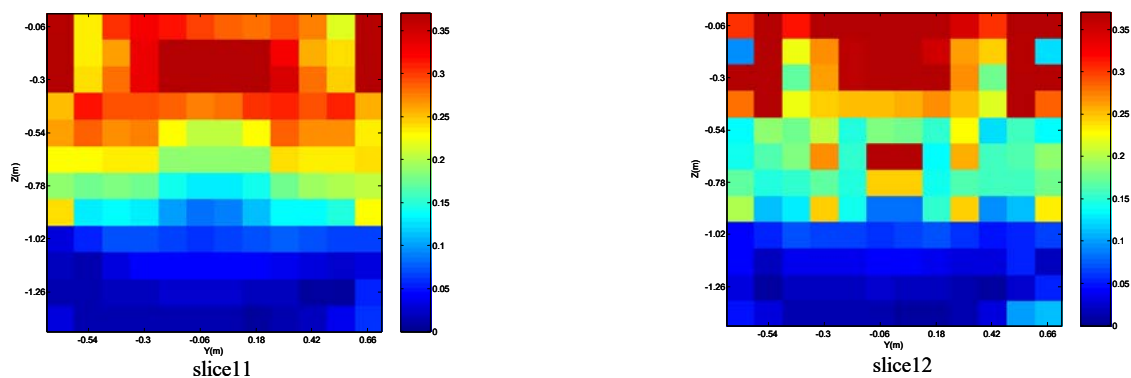
Figure 6: Inversion results, vertical slices 1-12, for a layered medium
